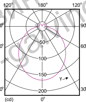
CLA LEDspotMV ND 5W PAR16 GU10 840 520lm
